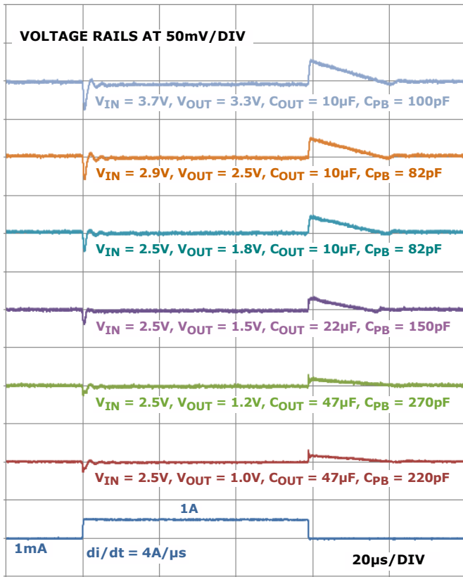
FIGURE 9. LOAD TRANSIENT WAVEFORMS
