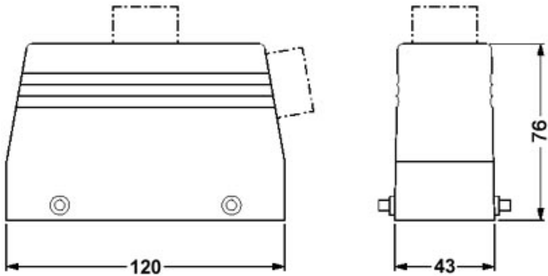
Dimensioned drawing
